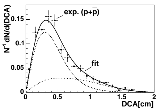
FIG. 2: DCA distribution for reconstructed proton tracks in the data sample (points with error bars). The result of the fit to the measured distribution (see text for more explanations) is denoted by the solid curve. The dashed (dashed-dotted) curve shows the contribution from primary (background) particles.
