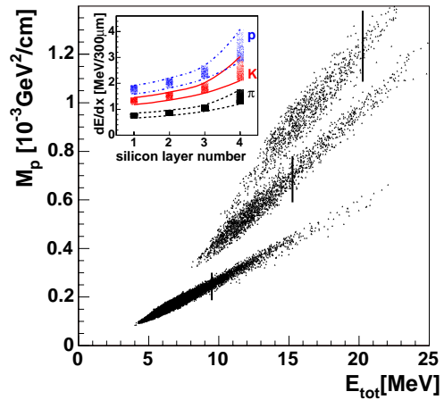
FIG. 1: (Color online) (M_p, E_{tot}) scatter plot for the candidate tracks after the (dE/dx)_i cuts in the first four spectrometer layers. Only track candidates with emission angles larger than 60^\circ are shown. The upper limits on E_{tot} are marked by vertical lines. An inset shows 1\sigma bands on the specific energy loss in the first four Si layers for simulated particles.
