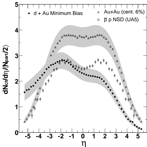
FIG. 2: dN_{ch}/d\eta distributions per participant are shown for minimum-bias d + Au collisions at \sqrt{s_{NN}} = 200 GeV (solid points), for central Au + Au collisions (0–6%) [12] (triangles) and for p + \bar{p} collisions from UA5 [19] (open squares) at the same energy. The systematic errors are shown by gray bands. The uncertainties on \langle N_{part} \rangle for d+Au and Au+Au collisions have been added in quadrature to the gray bands.
