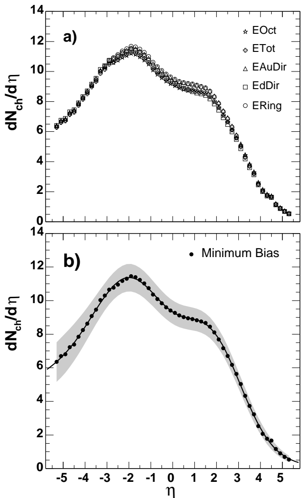
FIG. 1: Minimum-bias pseudorapidity distributions of primary charged particles, dN_{\text{ch}}/d\eta , measured for d + \text{Au} collisions at \sqrt{s_{NN}} = 200 GeV. a) dN_{\text{ch}}/d\eta distributions obtained by explicit integration over centrality bins for each centrality measure. b) Final dN_{\text{ch}}/d\eta distribution obtained by averaging over the five minimum-bias distributions. The gray band corresponds to the systematic errors (90% C.L.). The curve corresponds to a triple Gaussian fit to d + \text{Au} collisions.
