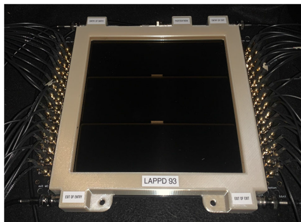
Fig. 1 Tile #93, fully cabled for the readout of 28 strips and to provide high voltage to the four MCPs and the photocathode. The sensitive area is about 380\text{ cm}^2
