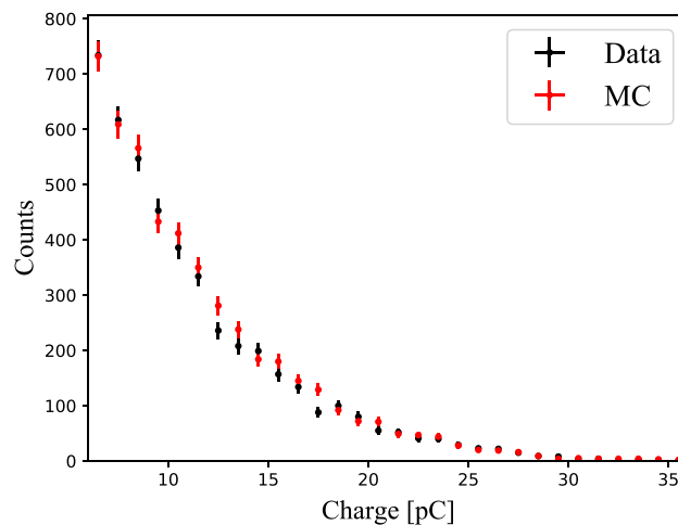
Fig. 6 Efficiency-calibrated trigger PMT charge distribution, in both data and MC, for a water target. The \chi^2/\text{ndf} comparing the data and MC is 22.9/30
