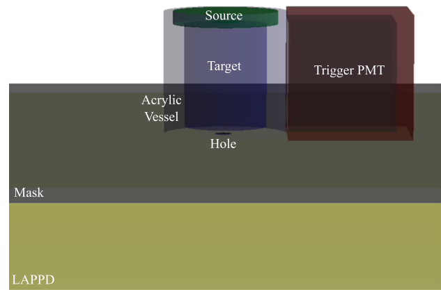
Fig. 4 The geometry of the setup, shown in Fig. 3, visualized looking from the side of the LAPPD in RAT-PAC
