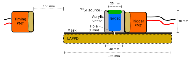
Fig. 3 The experimental setup used for the measurements in this paper. A ^{90}\text{Sr} \beta^- source is deployed above a liquid target contained in a cylindrical UVT acrylic vessel, above an LAPPD which is used to detect single photons, which are mostly blocked by a black mask. A PMT located \sim 25 cm away simultaneously detects single photons. An identical PMT is optically coupled to the acrylic vessel and used as trigger
