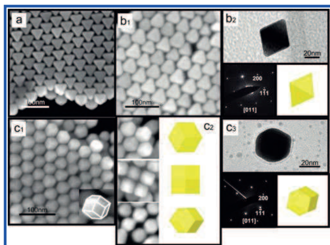
Figure 3. SEM images showing typically ordered assemblies of Au NPs prepared (a) without adding both HCl and \text{AgNO}_3 ( \{111\} -facet-bounded octahedral NPs, OC) and (b 1 ) with adding HCl but no \text{AgNO}_3 (OC). (b 2 ) TEM image, diffraction pattern, and model of an octahedron in sample (b 1 ). (c 1 ) SEM images of Au NPs prepared with adding \text{AgNO}_3 but no HCl ( \{110\} -facet-bounded rhombic dodecahedral NPs, RD). The inset shows an overview of a single NP. The frame scale of the inset is 50 nm. (c 2 ) Local SEM images and models of the RD NPs in various orientations. The frame scale of the inset is 100 nm. (c 3 ) TEM image, diffraction pattern, and model of a RD NP in sample (c 1 ).
