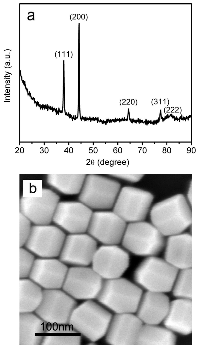
Figure S1. (a) XRD pattern of the Au nanocrystals with truncated ditetragonal prism (TDP) shape shown in Fig.1; (b)SEM image of larger Au TDP NPs (edge length of 72\pm 8\text{nm} ) synthesized by adding the equivalent of 0.25\mu\text{L} of the non-diluted seed solution.
