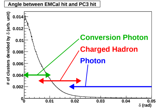
Figure 3.22: The distribution of \delta . Entry in each bin is divided by \delta . The distribution is roughly divided into 3 regions as displayed in the figure. The region of charged hadrons is discarded in the analysis.
