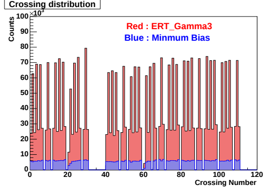
Figure A.26: Crossing distribution for the run corresponding to Figure A.25. Red histogram is for the ERT events and blue one is for the MB events.
