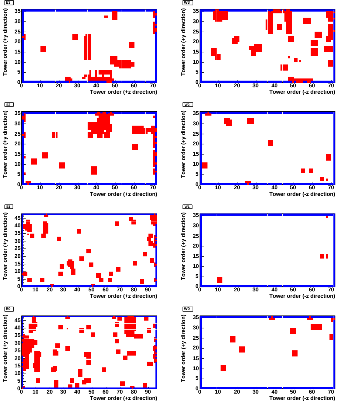
Figure 3.20: The masked towers. Eight histograms correspond to EMCAL sectors. The horizontal axis is the order of the tower parallel (antiparallel) to the beam axis in the east (west) arm. The vertical axis is the order of the tower along the y-axis. The red towers correspond to the warn towers and blue towers are edge towers. Both red and blue towers are masked in the analysis.
