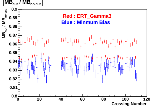
Figure A.25: The crossing dependence of the vertex cut efficiency for a certain run. Red points are for the ERT events and blue points are for the MB events.
