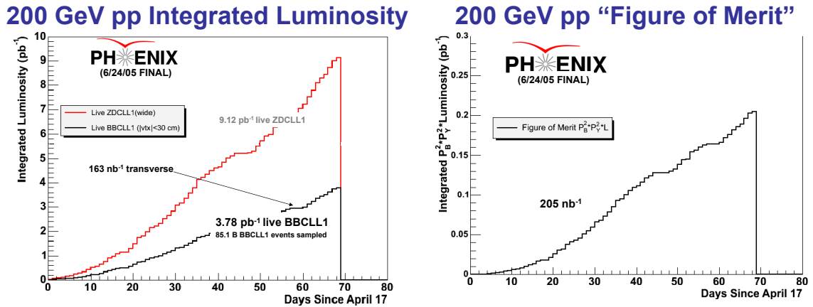
Figure 2.1: (Left) Integrated luminosity as a function of time. The black line is for BBCLL1 live trigger and the red line is for ZDCLL1-wide live trigger. Events with BBCLL1 is used in the usual analysis at PHENIX, as well as in this thesis. See Section 2.3.5 about the triggers. (Right) Figure-of-merit for A_{LL} as a function of time. The figure-of-merit is based on BBCLL1 live trigger. See Section 1.11 about the figure-of-merit.
