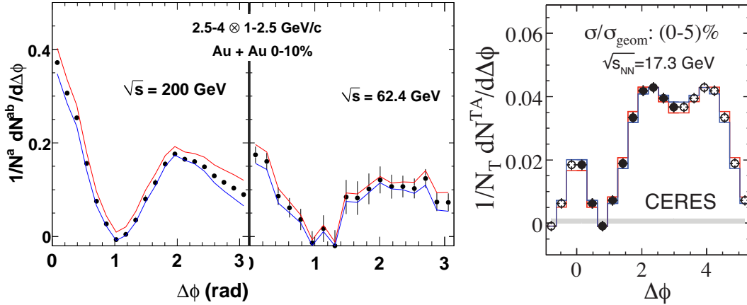
Figure 5.28: Survey of jet per-trigger yields by beam energy: Central Au+Au at \sqrt{s_{NN}}=200 and 62.4 GeV within \eta = \pm 0.35 at PHENIX [53] (left) and central Pb+Au at \sqrt{s_{NN}}=17.3 GeV within 0.1 < \eta < 0.7 at CERES [100] (right).
