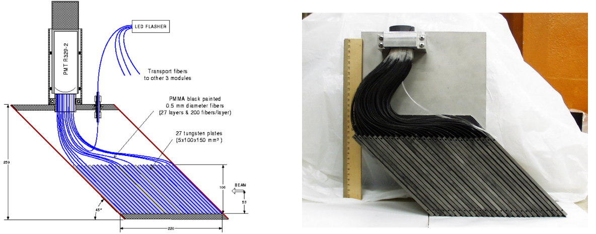
Figure 3.6: (Left) Schematic of a ZDC module. (Right) A photo of a ZDC module.
