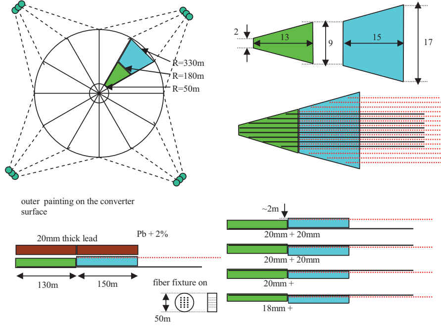
Figure 3.7: Schematic view of the Reaction Plane Detector
