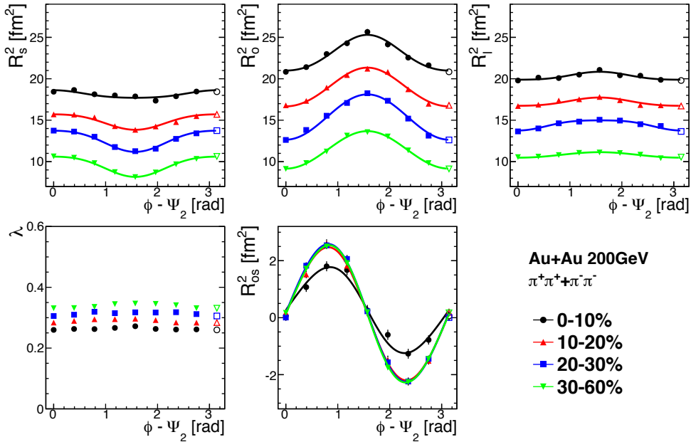
Figure 5.10: Extracted HBT parameters of charged pions in 0.2 < k_T < 2.0 GeV/ c as a function of azimuthal pair angle with respect to 2 nd -order event plane for four centrality bins. The data point at \Delta\Phi = \pi is same value at \Delta\Phi = 0 . Solid lines depict fit functions by Eq. (5.1).
