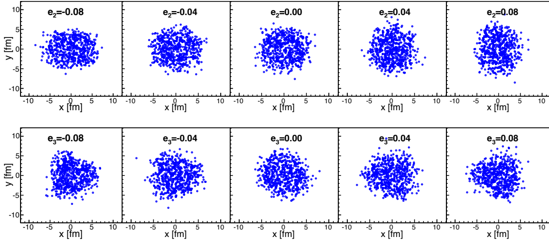
Figure 6.23: Scatter plots of generated particles in x - y plane for elliptical ( n=2 ) and triangular ( n=3 ) source, where R_0 = 5 fm, a = 0.54 .
