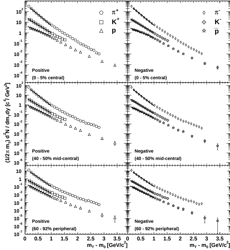
Figure 1.6: Transverse mass m_T distributions for \pi^\pm , K^\pm , p(\bar{p}) for 3 centrality bins in Au+Au collisions at \sqrt{s_{NN}}=200 GeV [12]. The solid lines on each spectra represent fitting results with m_T exponential function.
