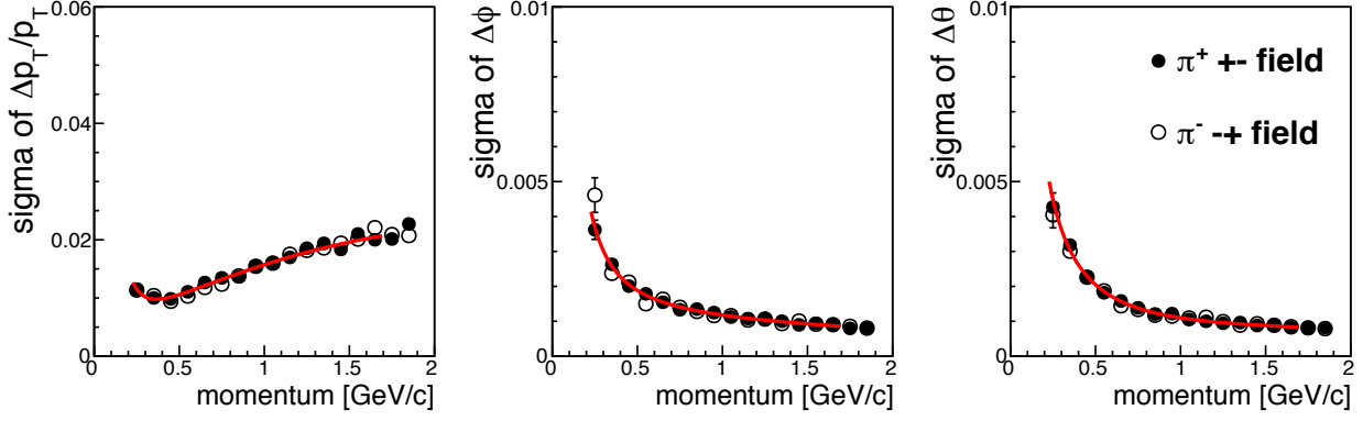
Figure 4.19: Momentum resolution for charged pions with polynomial fit. The standard deviations of \Delta p_T/p_T , \Delta\phi , \Delta\theta distribution obtained by the Gaussian fit are plotted as a function momentum.
