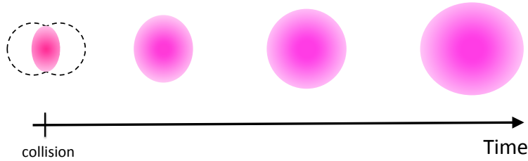
Figure 1.14: A sketch of the evolution of the system shape in coordinate space after the collision.
