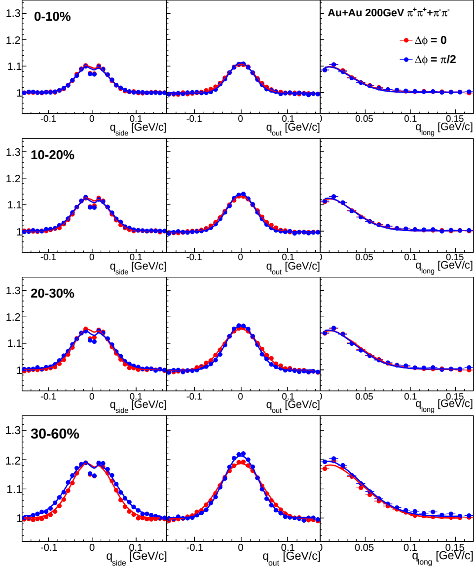
Figure A.13: Projected 3D correlation functions of charged pion pairs measured with respect to 2^{\text{nd}} -order event plane for 0.2 < k_T < 2.0 GeV/c with the correction of the event plane resolution. Correlation functions at \Delta\phi = 0 (red symbol) and \Delta\phi = \pi/2 (blue symbol) are shown. Correlation functions are projected along each q directions with q_{\text{other}} < 50 [MeV/c]. Solid lines show the fit functions.
