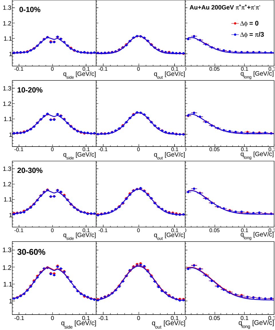
Figure A.19: Projected 3D correlation functions of charged pion pairs measured with respect to 3 rd -order event plane for 0.2 < k_T < 2.0 GeV/c at four centrality bins without the correction of the event plane resolution. Correlation functions at \Delta\phi = 0 (red symbol) and \Delta\phi = \pi/3 (blue symbol) are shown. Correlation functions are projected along each q directions with q_{other} < 50 [MeV/c]. Solid lines show the fit functions.
