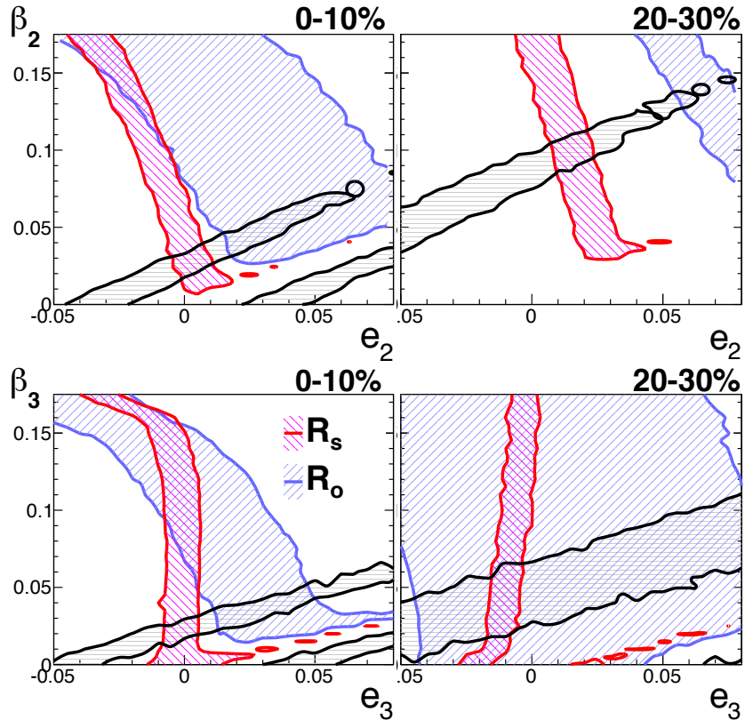
Figure 6.38: Contour map of \chi^2 between data and simulation for 2 nd - and 3 rd -order, where the \chi^2 is calculated from the relative amplitudes of R_o and R_s , and v_n . Shaded areas represent the regions within 2\sigma contour for 2 nd -order HBT and 1\sigma contour for 3 rd -order HBT, and 4\sigma contour for v_n .
