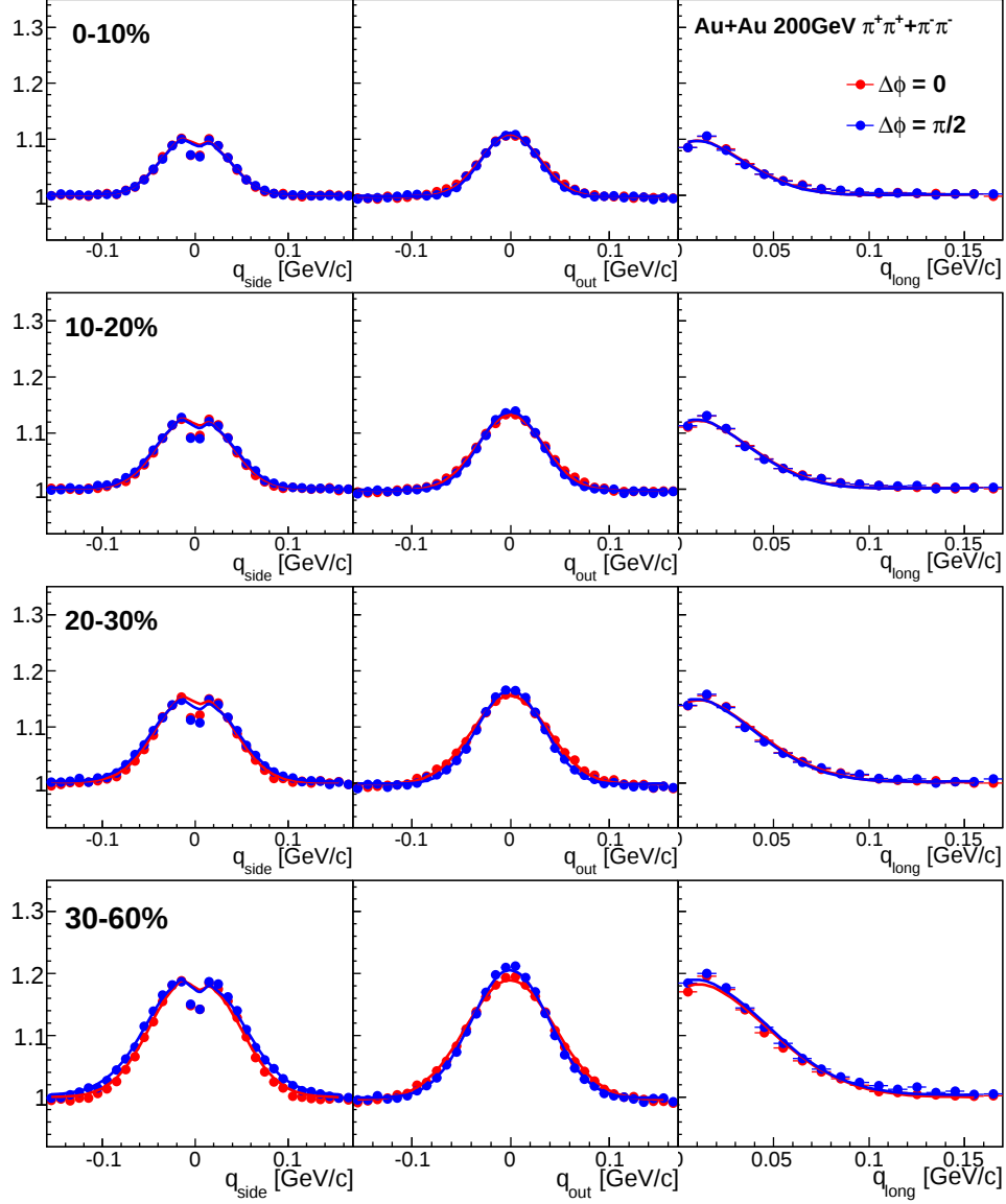
Figure 5.8: Projected 3D correlation functions of charged pion pairs in 0.2 < k_T < 2.0 GeV/ c at four centrality bins without the correction of the event plane resolution. Correlation functions at \Delta\phi = 0 (red symbol) and \Delta\phi = \pi/2 (blue symbol) are shown. Correlation functions are projected along each q directions with q_{other} < 50 [MeV/ c ]. Solid lines show the fit functions by Eq. (4.36), which is also projected in the same way.
