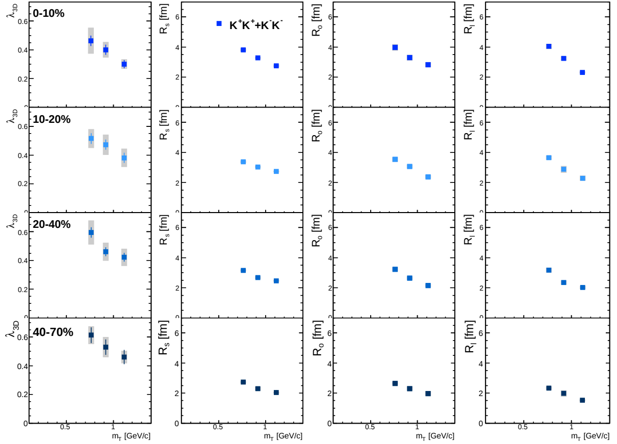
Figure 5.5: 3D HBT parameters of charged kaons as a function of m_T for four centrality bins, where positive and negative kaon pairs are combined.
