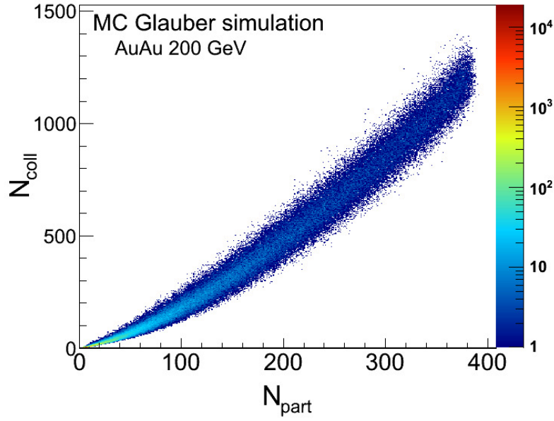
Figure 6.12: Number of binary collisions ( N_{coll} ) vs number of the participant nucleons are plotted for AuAu collisions at 200 GeV from MC Glauber simulation.
