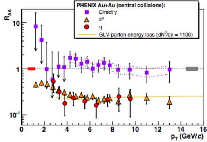
Figure 1.11: The nuclear modification factor ( R_{AA}(p_T) ) measured in central Au+Au at colliding energy 200 GeV for \pi^0 , \eta and direct photon [31].
