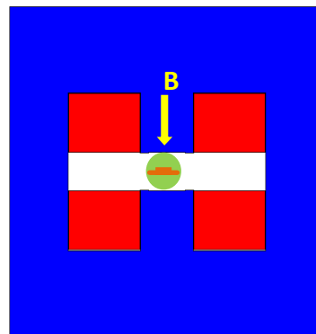
Figure 2: Top view of the magnet and sample holder. Field angle zero is defined as perpendicular to the tape surface.
