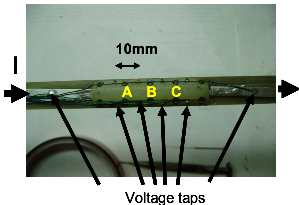
Figure 4: A photograph of a sample holder with 4mm YBCO tape and 10mm segments "A", "B" and "C" irradiated. A 4mm wide YBCO sample is placed under the G-10 cover. The position of voltage taps is shown. The direction of current is shown as left to right arrow.
