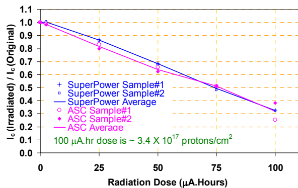
Figure 1 Normalized critical current versus radiation for self-field.
