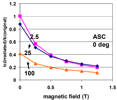
Figure 10: Normalized critical current versus magnetic field at zero degree position for ASC samples.
