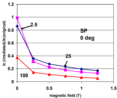
Figure 9: Normalized critical current versus magnetic field at zero degree position for SuperPower sample.
