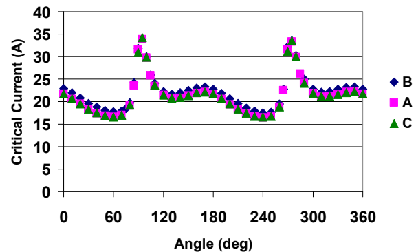
Figure 5: Critical Current at different sections at the same magnetic field (0.5 T) at a low dose level (2.5 \mu\text{A}\cdot\text{hr} ) for SuperPower samples.
