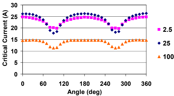
Figure 8: Critical current versus angle for YBCO from ASC at 1.0T, 77K
