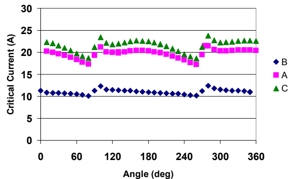
Figure 6: Critical current at three different sections at 0.5T at a high dose level (100 \mu\text{A}\cdot\text{hr} ) for SuperPower samples
