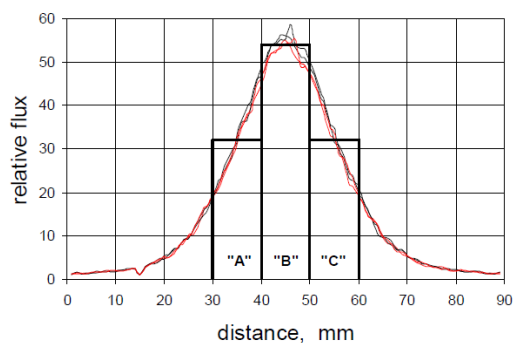
Figure 3: The position of the three 10mm segments in the beam cross section.
