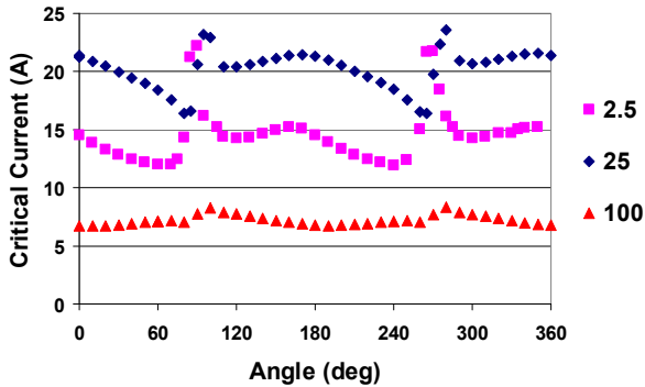
Figure 7: Critical current versus angle for YBCO from SuperPower at 1.0T, 77K
